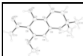
Fig. 1. View of the title compound with displacement ellipsoids drawn at the 30% probability level.
